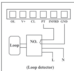
Loop Detector NO
