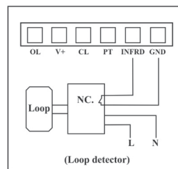
Loop Detector NC
